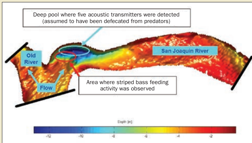
Figure 6-18 Plan-view, bathymetry of the Old River/San Joaquin River flow split (bathymetry graphic courtesy of Jon Burau and Aaron Blake, USGS).
