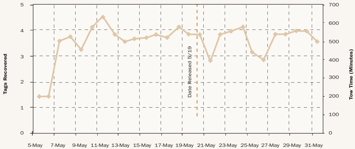
Appendix C-4, Figure 9 Antioch/Mosssdale 2
