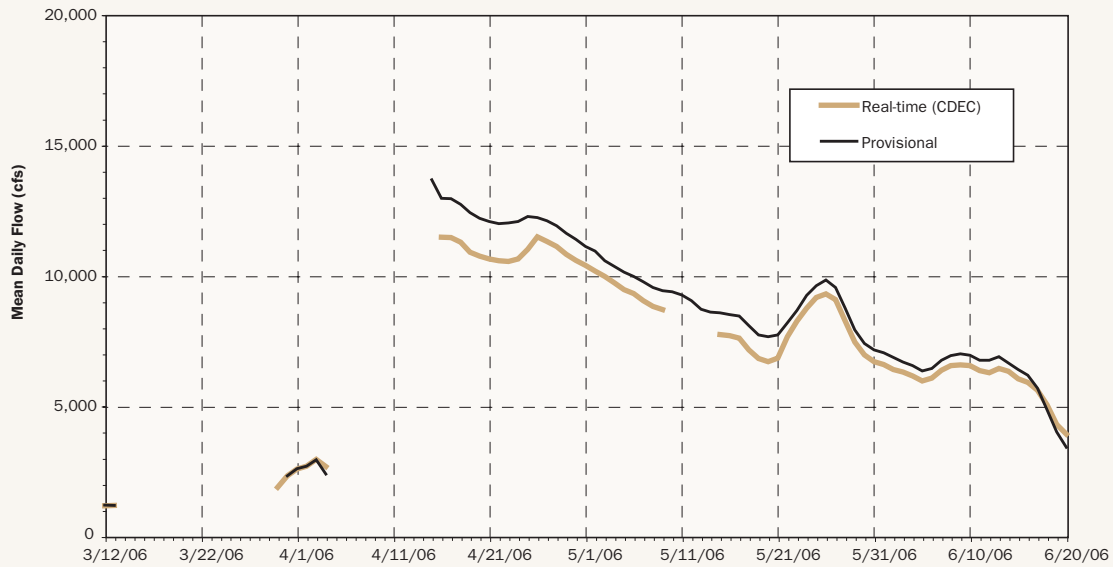
Appendix A-2, Figure 3 San Joaquin River above Merced River
