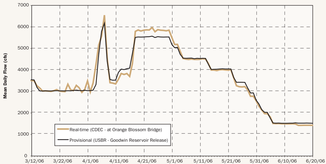
Appendix A-2, Figure 6 Stanislaus River below Goodwin Dam
