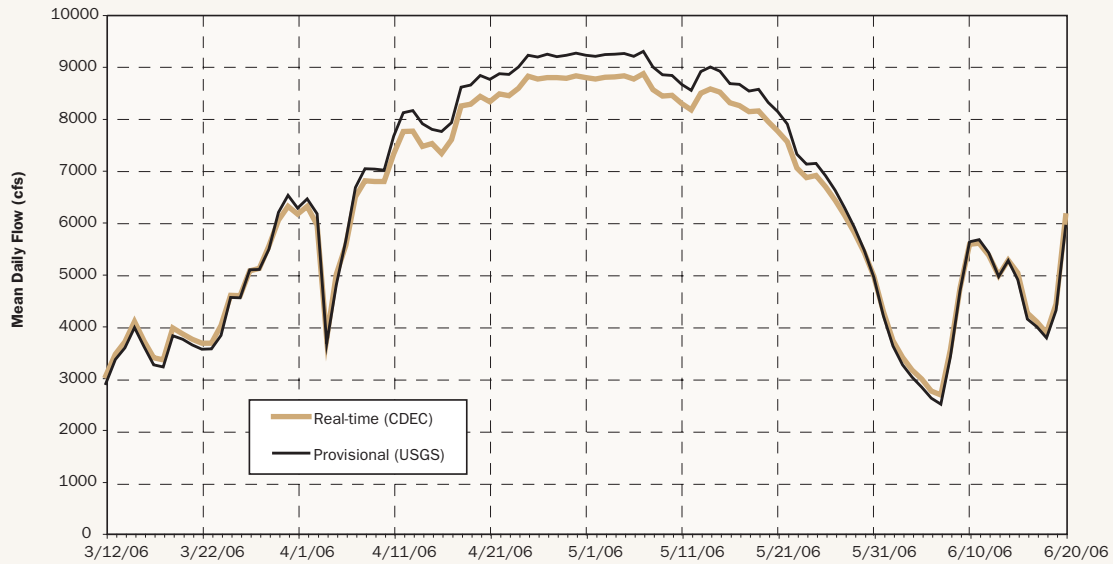
Appendix A-2, Figure 5 Tuolumne River below LaGrange Dam
